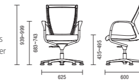
T503FFGFU swivel communication chair with upgraded structure and materials
